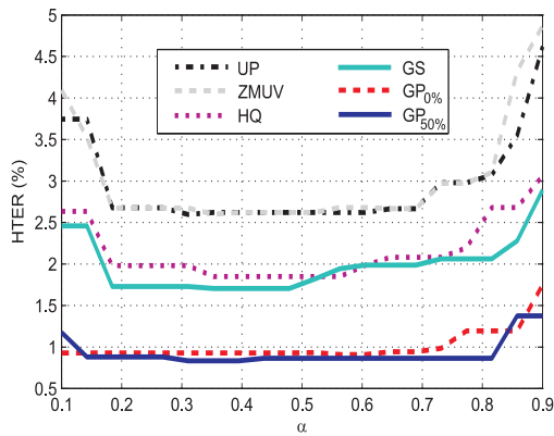
Figure 5. EPC curves obtained on the test image set Slika 10. EPC krivulje poizkusov na testnem delu zbirke PolyU
