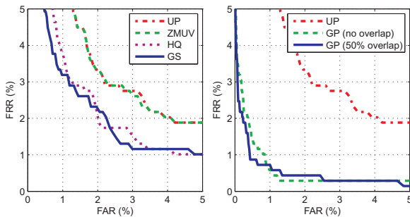
Figure 4. ROC curves of the experiments Slika 9. ROC krivulje poizkusov
